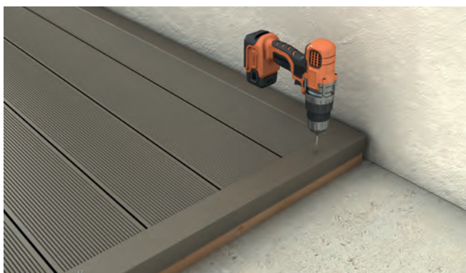
Fix colour-coded Edging Trim using Ø3mm stainless steel screws at 500mm centres.
