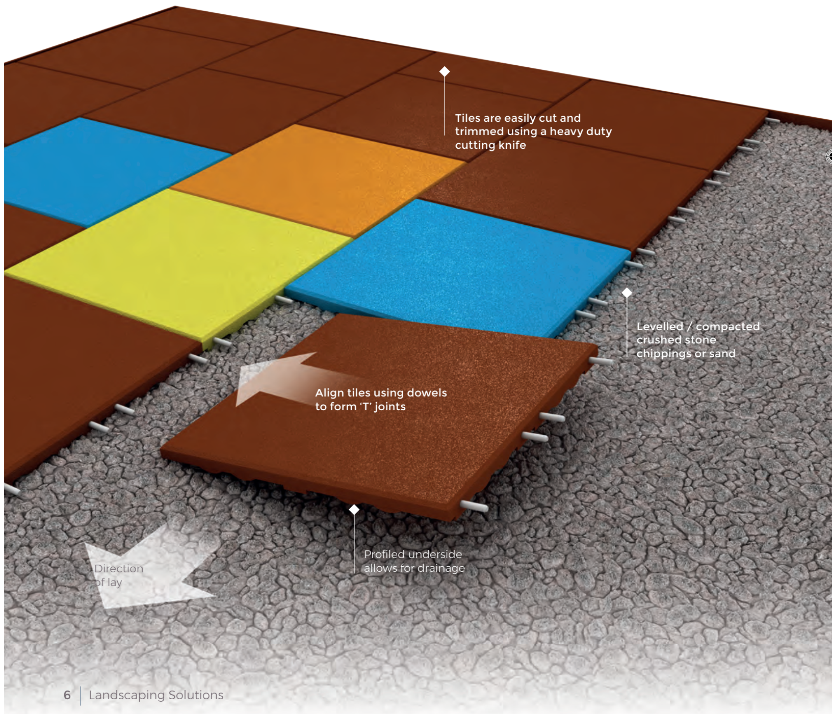
Correct 'T' joint laydown
