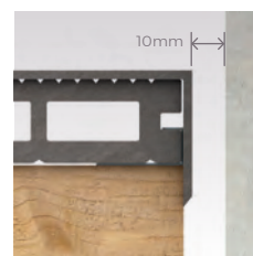
Provide a minimum 10mm gap between edge of decking and any adjacent wall.
