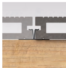
DuraDek stainless steel joint clip provides secure fit and even spacing of planks.
