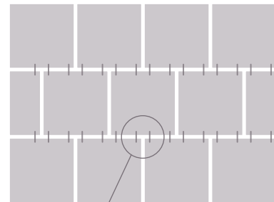
Correct 'T' joint laydown
