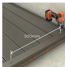
Fix colour-coded Edging Trim using Ø3mm stainless steel screws at 500mm centres.
